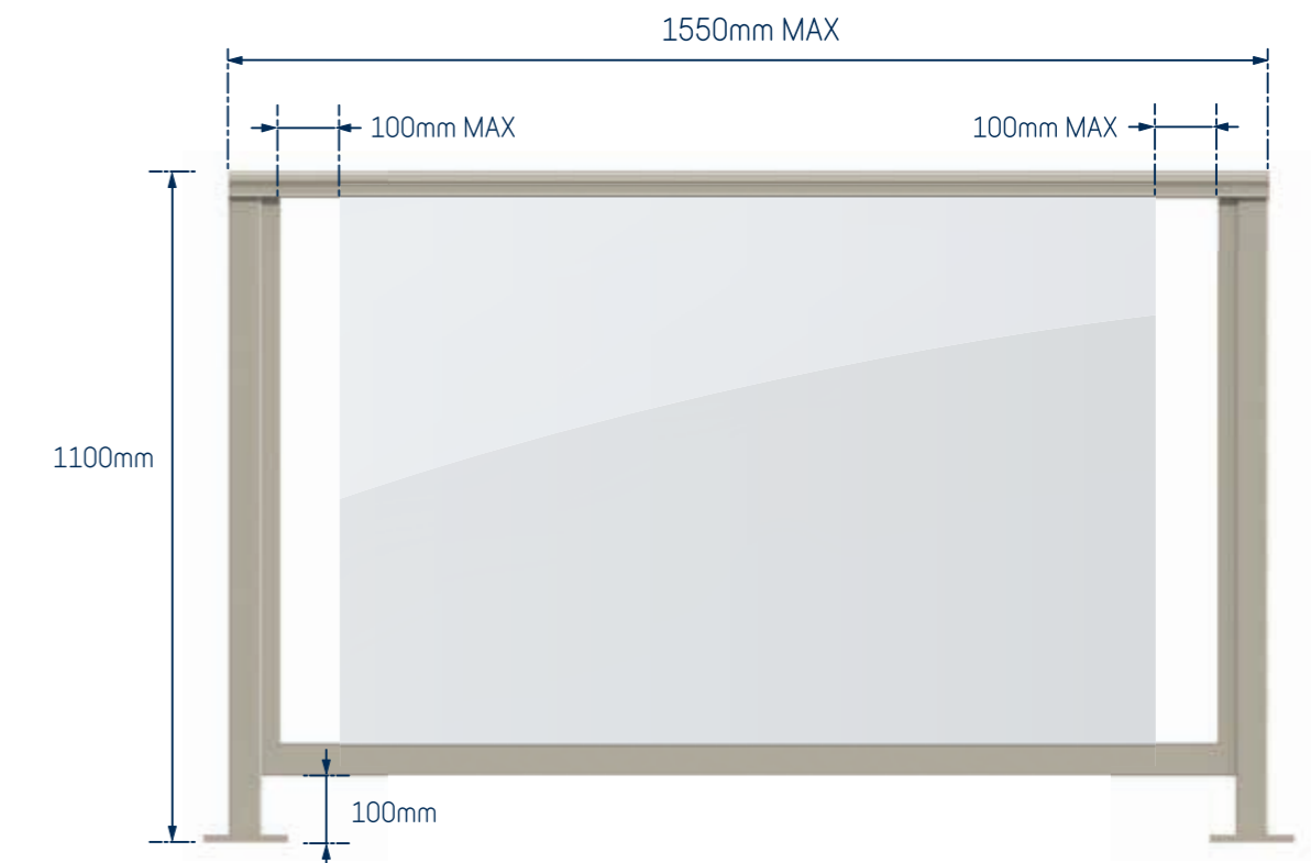
BALUSTRADE VERTICAL GLAZING
